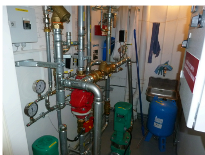
Sprinkler panel
